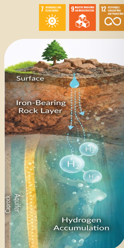
Geological cross-section of natural hydrogen generation via water–rock reactions and subsurface accumulation.
