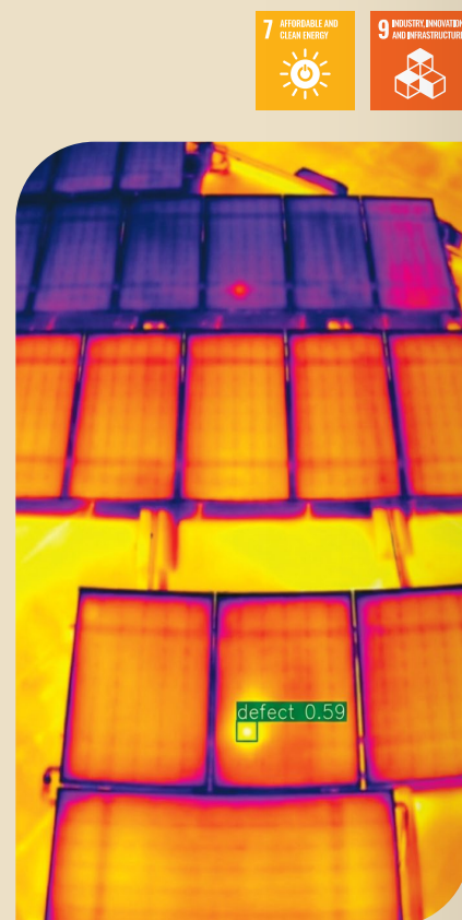
Thermal infrared imaging of solar panels with AI-detected faults for performance monitoring.
